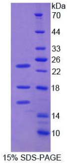
Figure 3. SDS-PAGE
