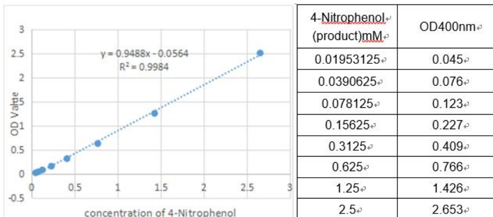
Figure 1. The standard curve of 4-Nitrophenol
