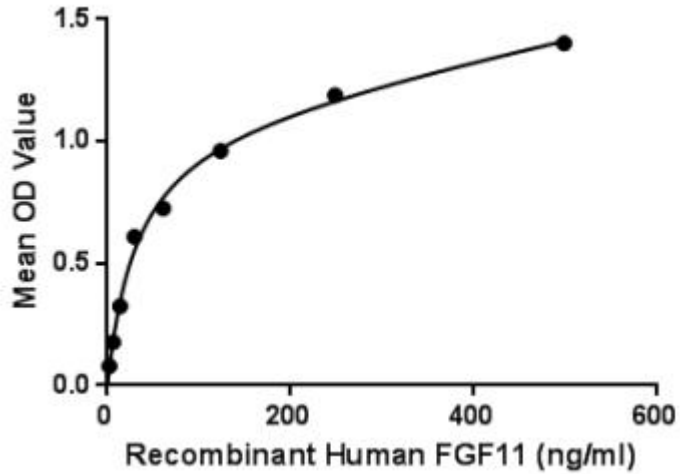
Figure 1. The binding activity of FGF11 with FGFR1
