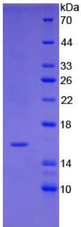
Figure 4. SDS-PAGE
