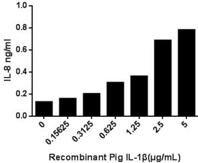
Figure1. IL-8 levels in the cell supernatant of A549 induced by IL-1 \beta
