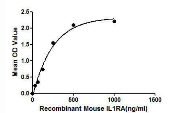
Figure 1. The binding activity of IL1RA with IL1R1.
