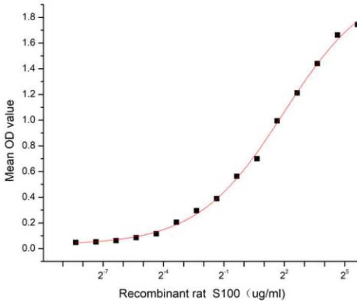
Figure 1. The binding activity of recombinant rat S100A1 and recombinant mouse S100A4
