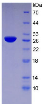
Figure 4. SDS-PAGE
