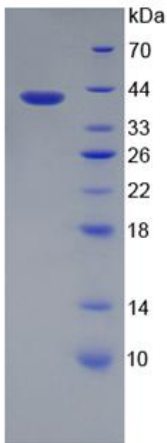
Figure 4. SDS-PAGE
