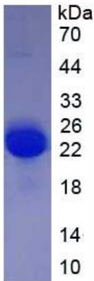
Figure 2. SDS-PAGE
