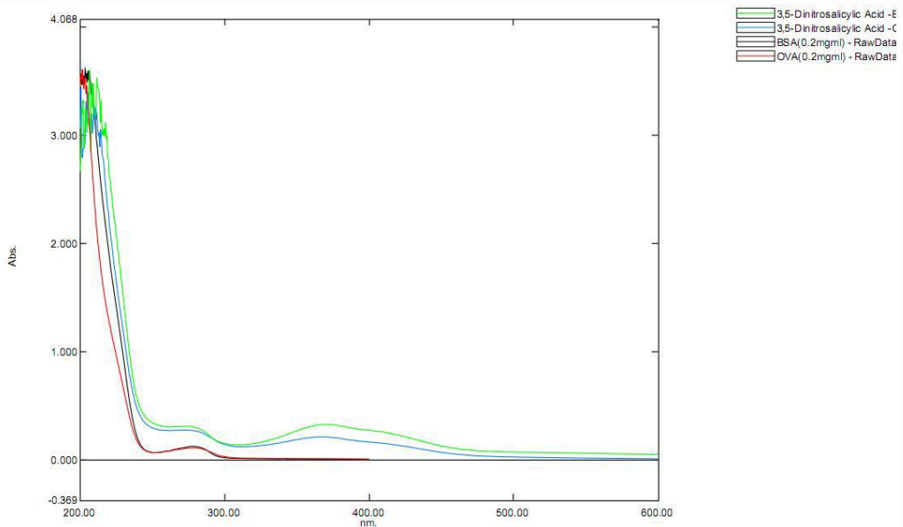
Figure 1. UV-spectrum
