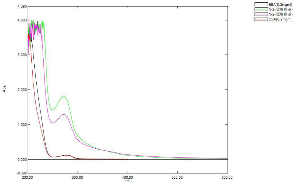
Figure 1. UV-spectrum
