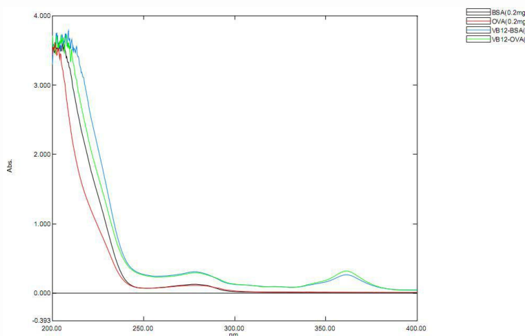
Figure 2. UV-spectrum
