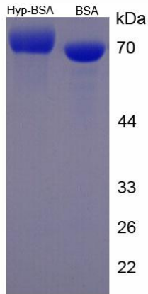
Figure 1. SDS-PAGE
