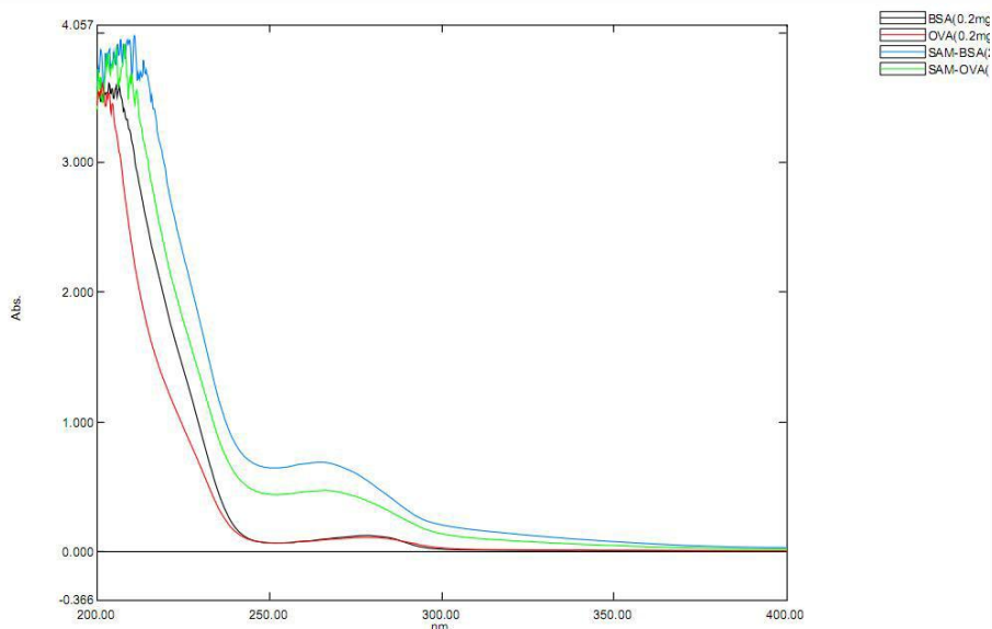
Figure 2. UV-spectrum
