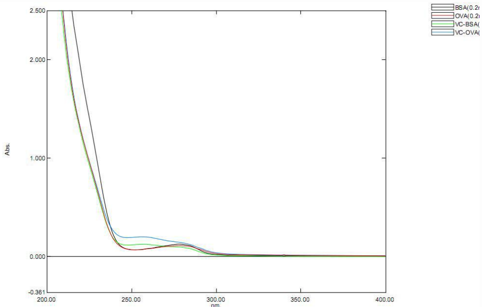
Figure 2. UV-spectrum
