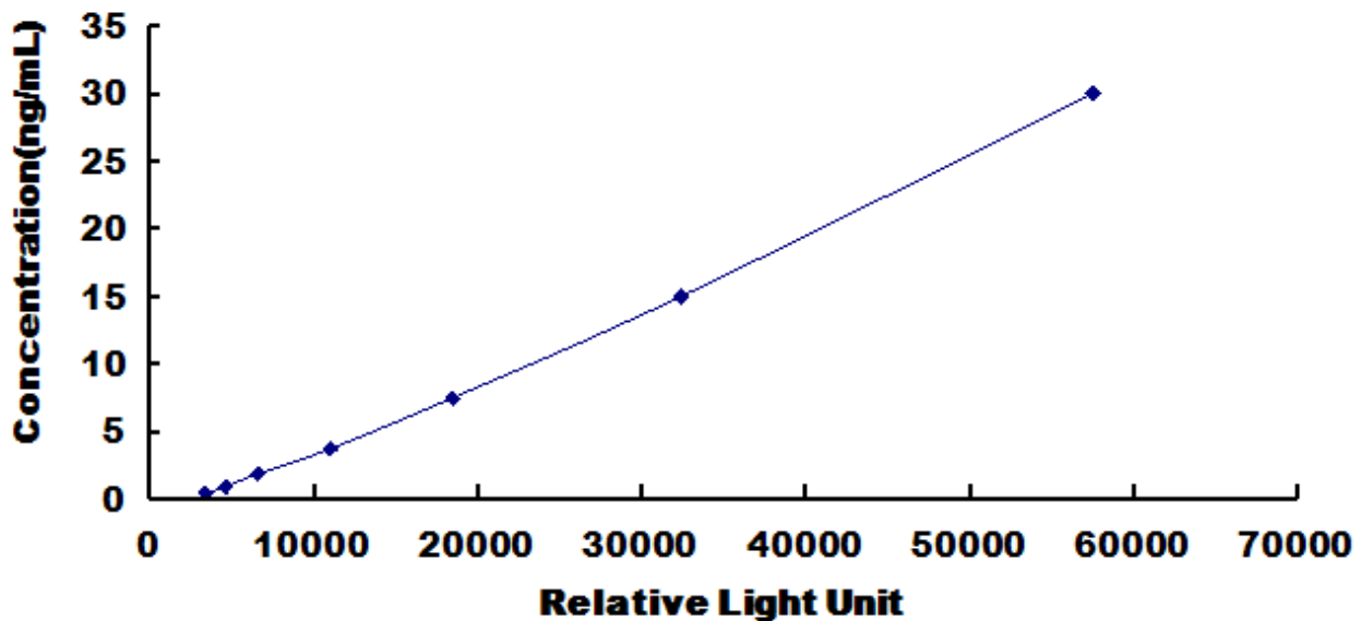
Typical Standard Curve for Human AGC CLIA.
