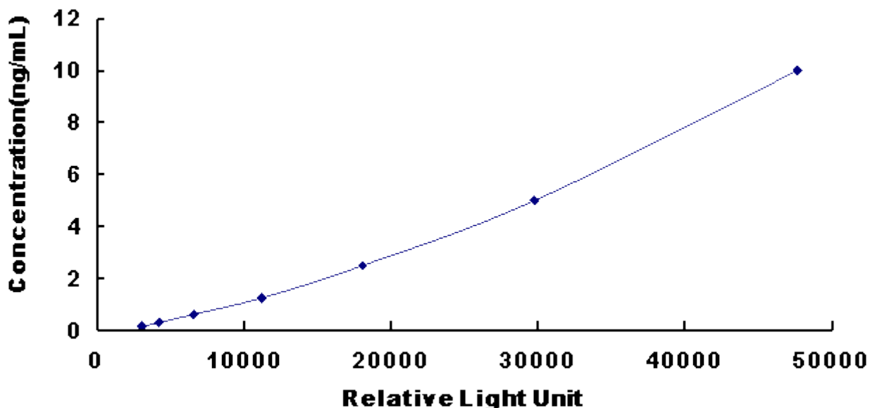
Typical Standard Curve for Mouse CCKAR CLIA.
