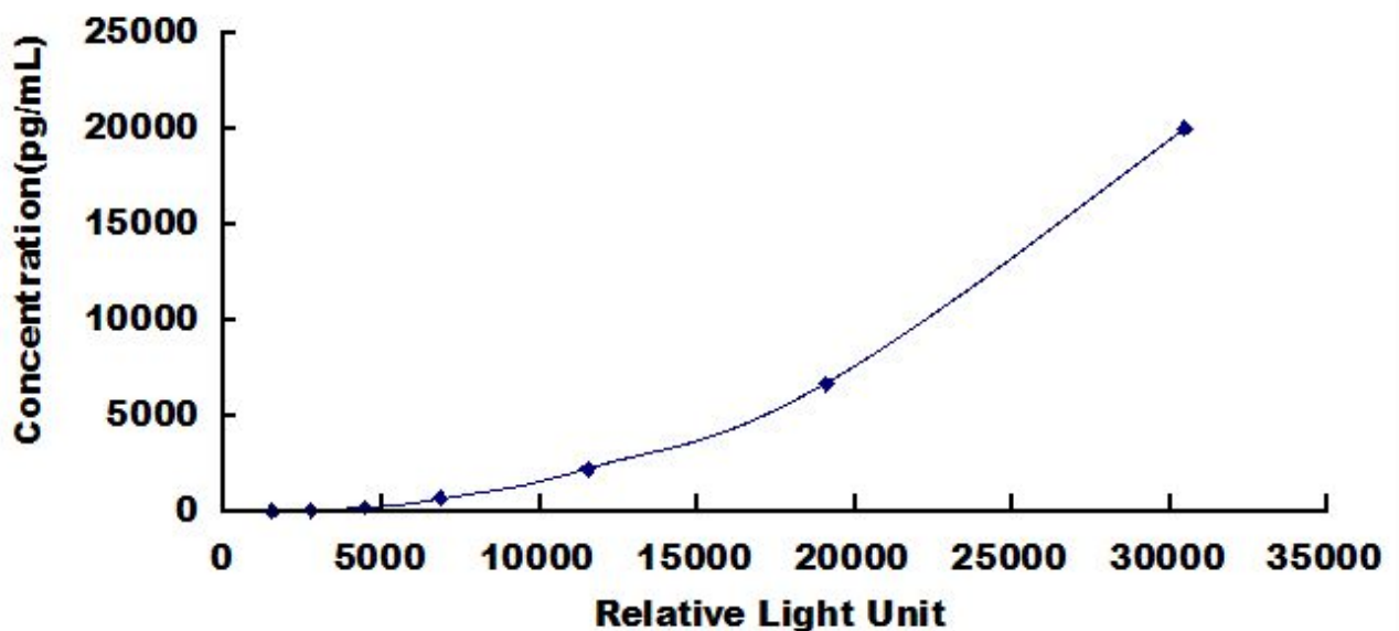
Typical Standard Curve for COL10, Human CLIA.
