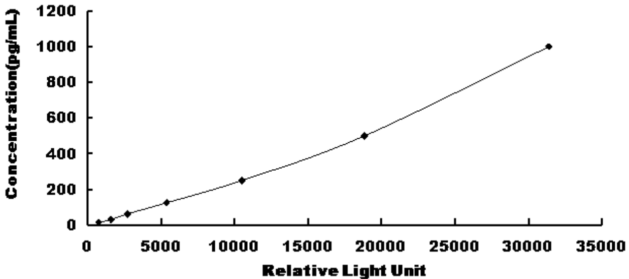
Typical Standard Curve for Mouse GCSF CLIA.
