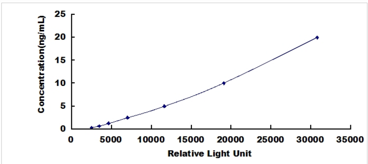
Typical Standard Curve for DEFa1, Human CLIA.
