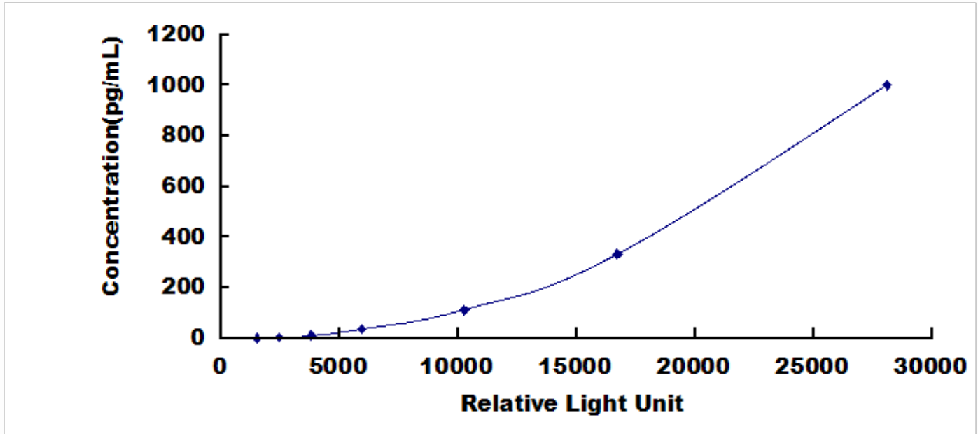
Typical Standard Curve for Epiregulin, Rat CLIA.
