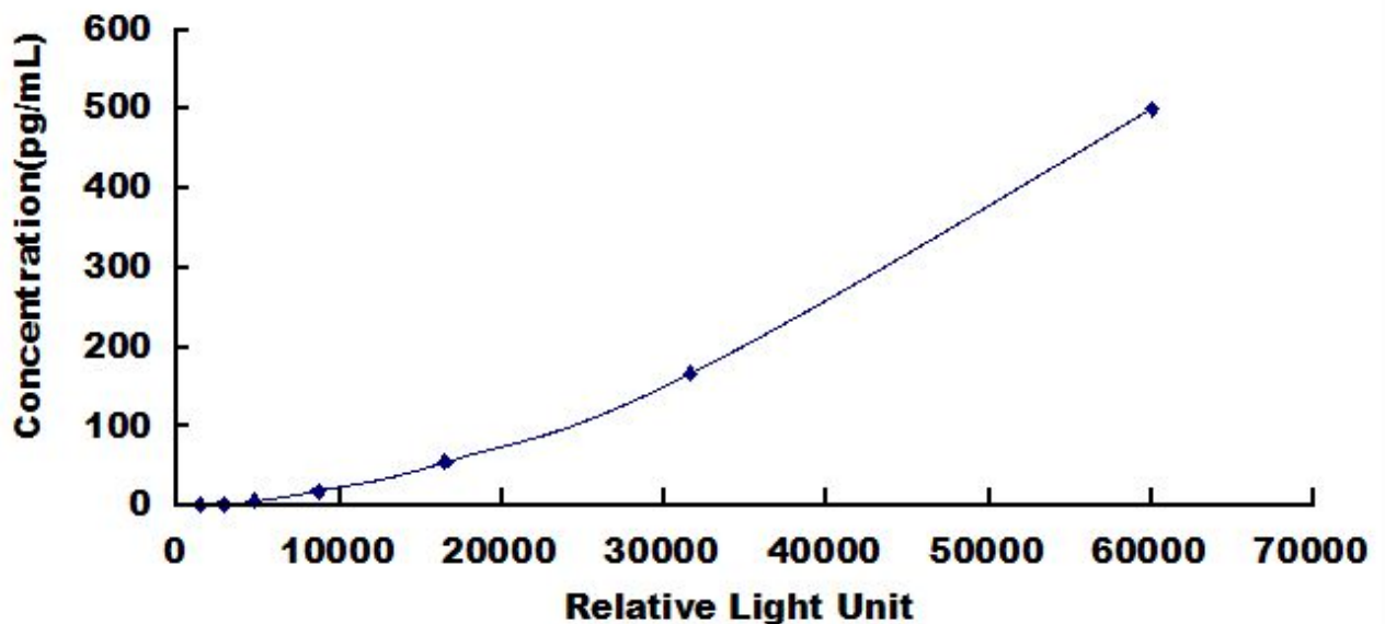
Typical Standard Curve for FGF13, Human CLIA.
