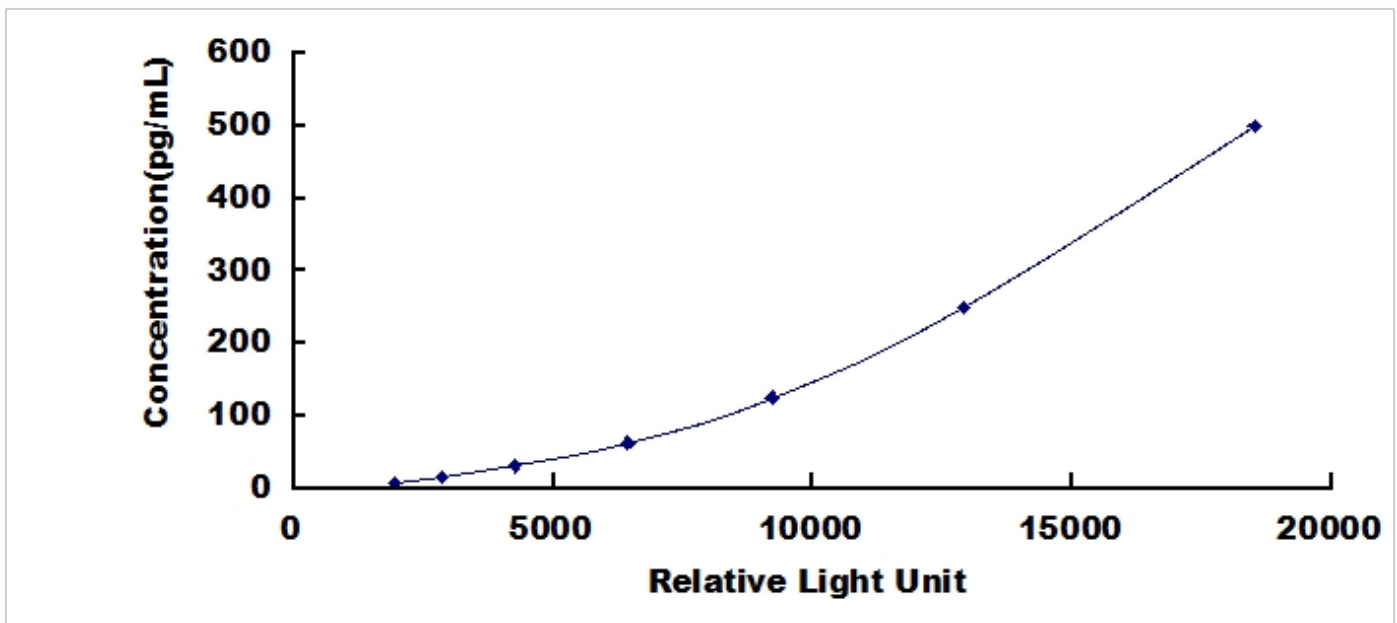
Typical Standard Curve for GAL9, Mouse CLIA.
