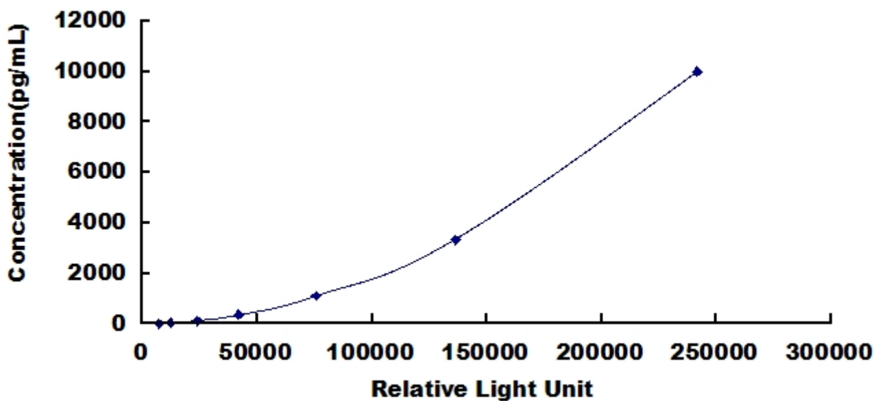
Typical Standard Curve for GDNF, Human CLIA.
