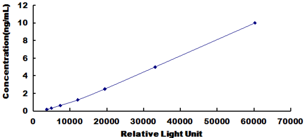
Typical Standard Curve for Gallus GH CLIA.
