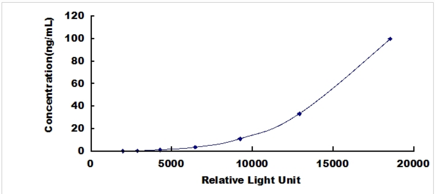
Typical Standard Curve for Hsp60, Mouse CLIA.
