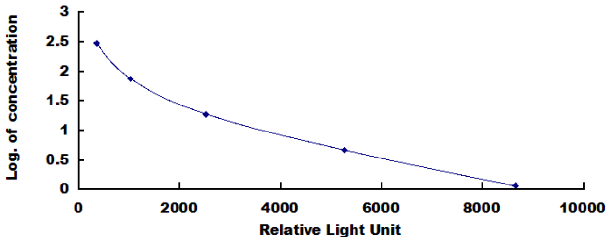
Typical Standard Curve for Hemoglobin, Human CLIA.
