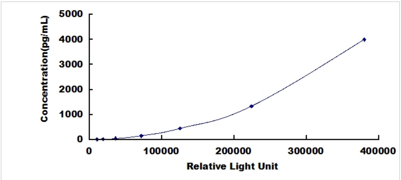
Typical Standard Curve for Hepcidin, Human CLIA.
