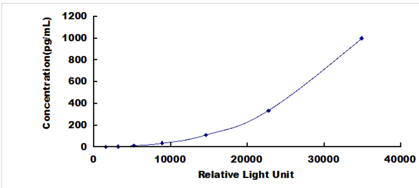
Typical Standard Curve for IFNg, Human CLIA.
