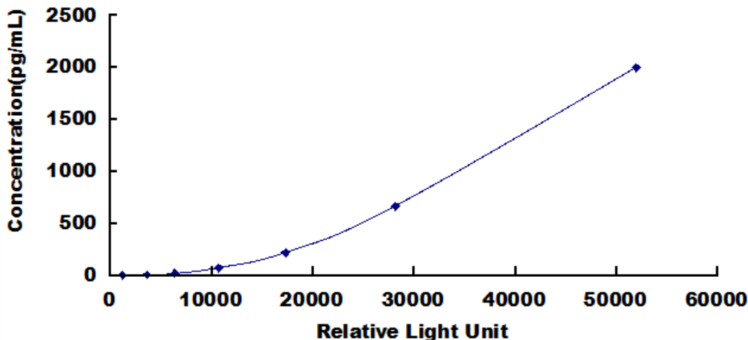
Typical Standard Curve for IL17, Mouse CLIA.
