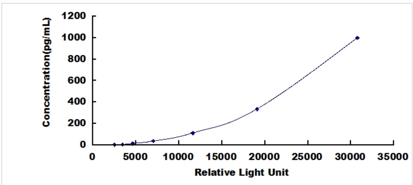
Typical Standard Curve for IL26, Human CLIA.
