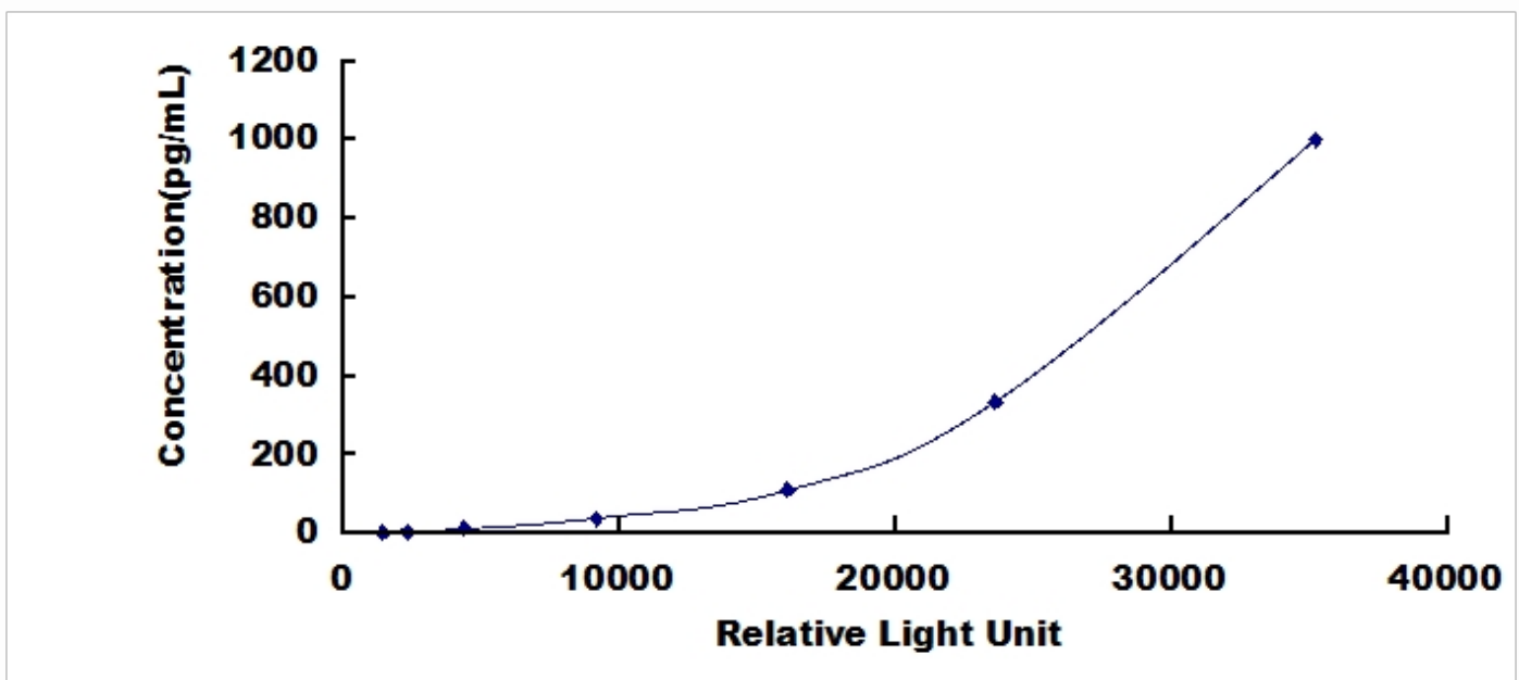
Typical Standard Curve for IL28B, Human CLIA.
