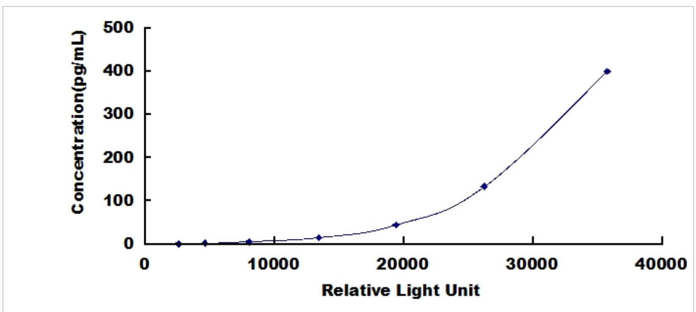
Typical Standard Curve for IL6, Mouse CLIA.
