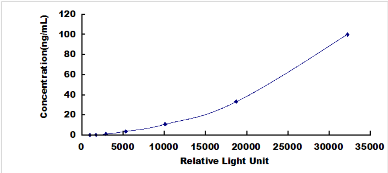
Typical Standard Curve for NAGase, Rat CLIA.
