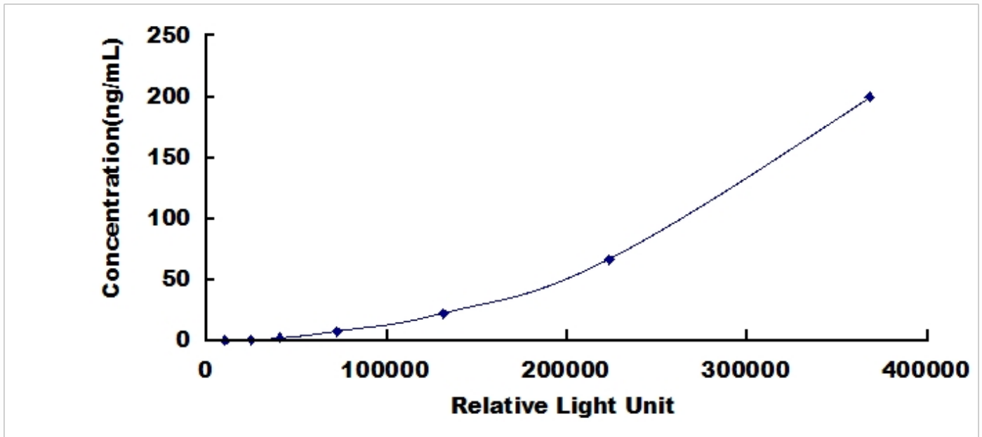
Typical Standard Curve for PARP, Human CLIA.
