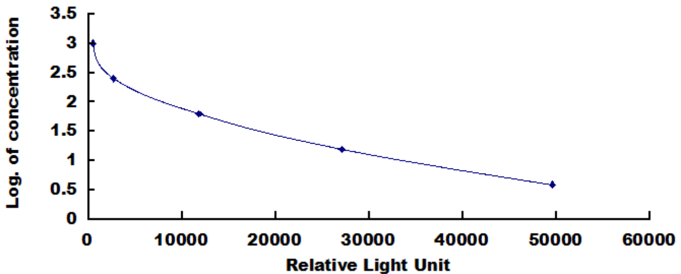
Typical Standard Curve for PEG CLIA.
