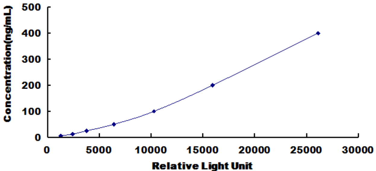
Typical Standard Curve for Human SAP CLIA.
