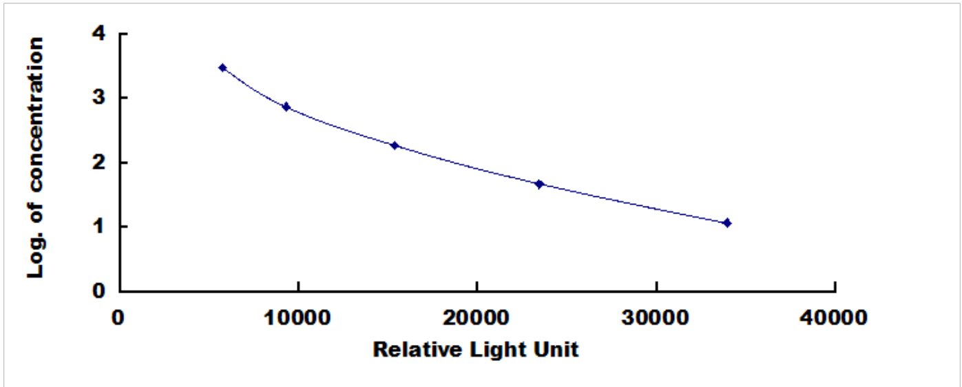
Typical Standard Curve for SP, Bovine CLIA.
