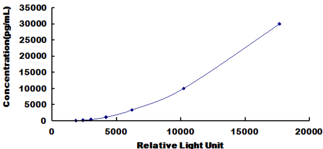
Typical Standard Curve for TrxR1, Human CLIA.
