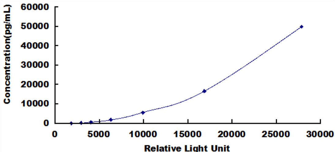
Typical Standard Curve for Thyroglobulin, Human CLIA.
