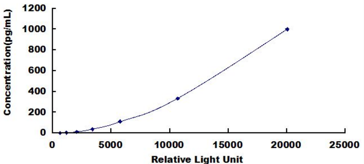
Typical Standard Curve for TGFb3, Porcine CLIA.
