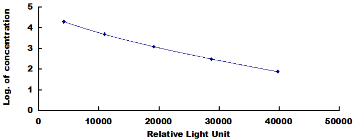
Typical Standard Curve for T3 CLIA.
