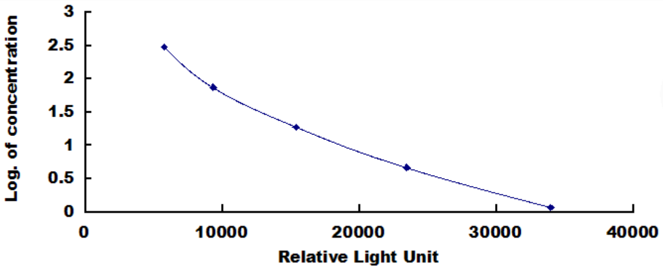
Typical Standard Curve for VB1 CLIA.
