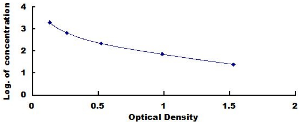
Typical Standard Curve of ELISA kit for Rat, CGRP.
