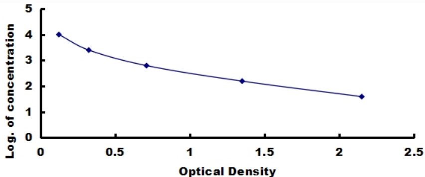
Typical Standard Curve of ELISA Assay for Rat, CTXI.
