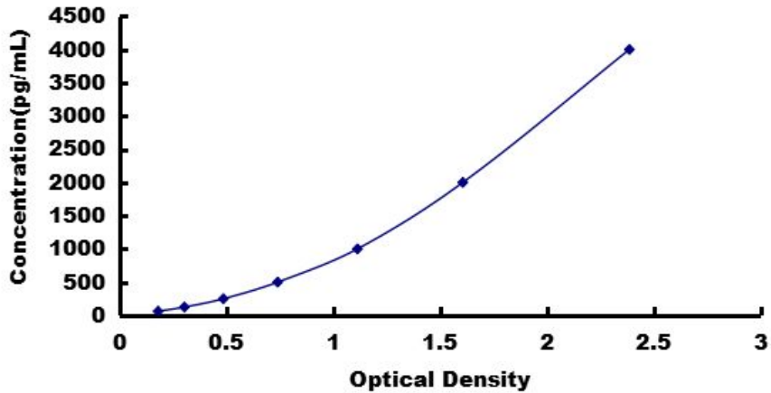
Typical Standard Curve of ELISA kit for Rat, FGF2.
