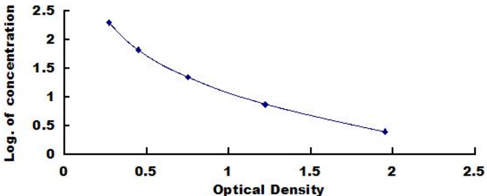
Typical Standard Curve of ELISA kit for Rat, Hepc.
