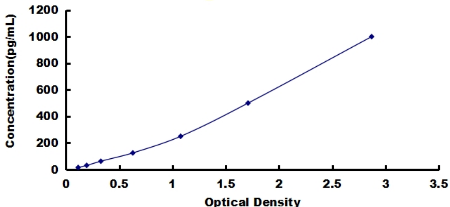
Typical Standard Curve of ELISA Assay for Rat, IL10.
