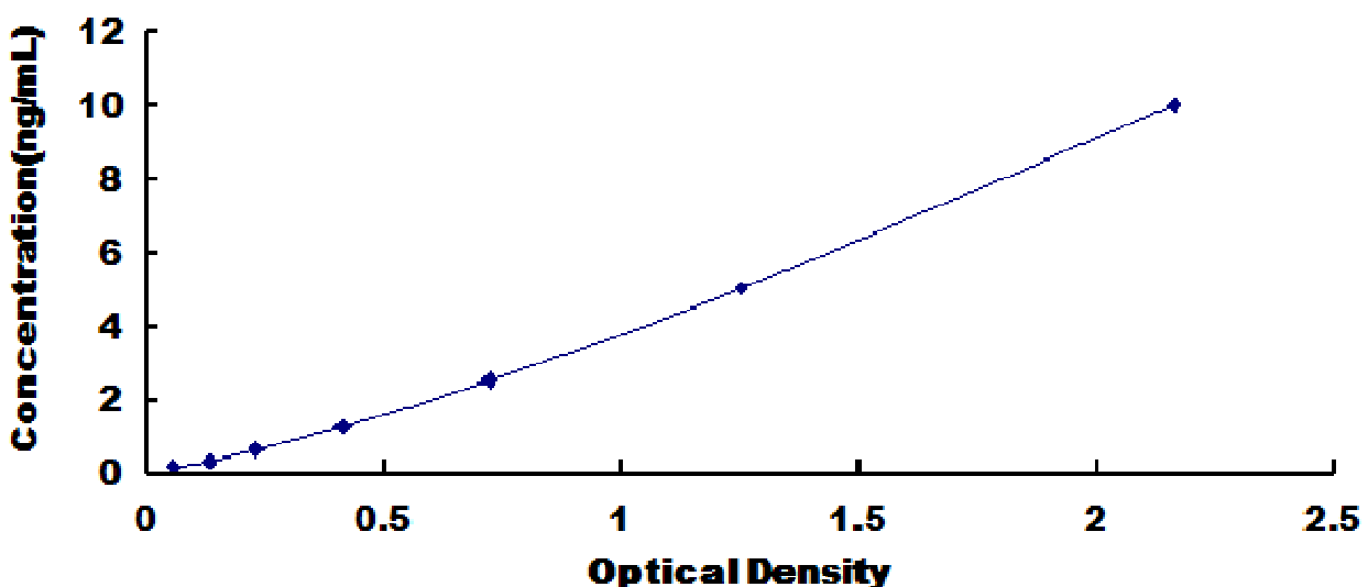
Typical Standard Curve for HSD17b10, Mouse ELISA.
